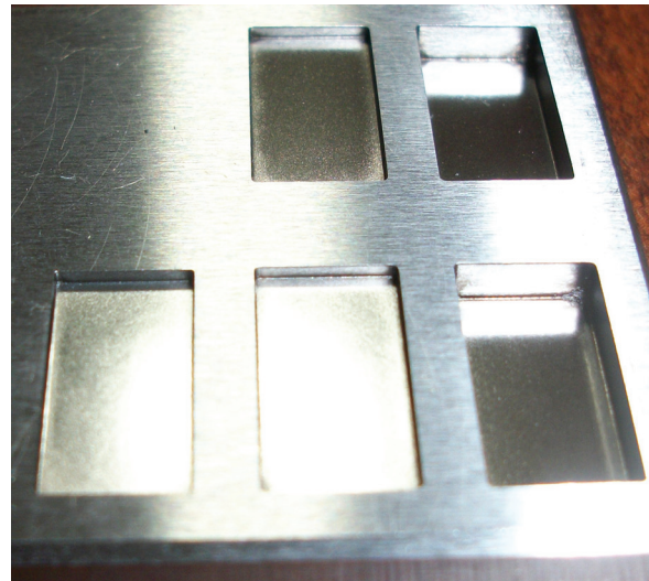
Figure 2. Fine surface finish available with an appropriate graphite electrode material and proper machine parameters.
